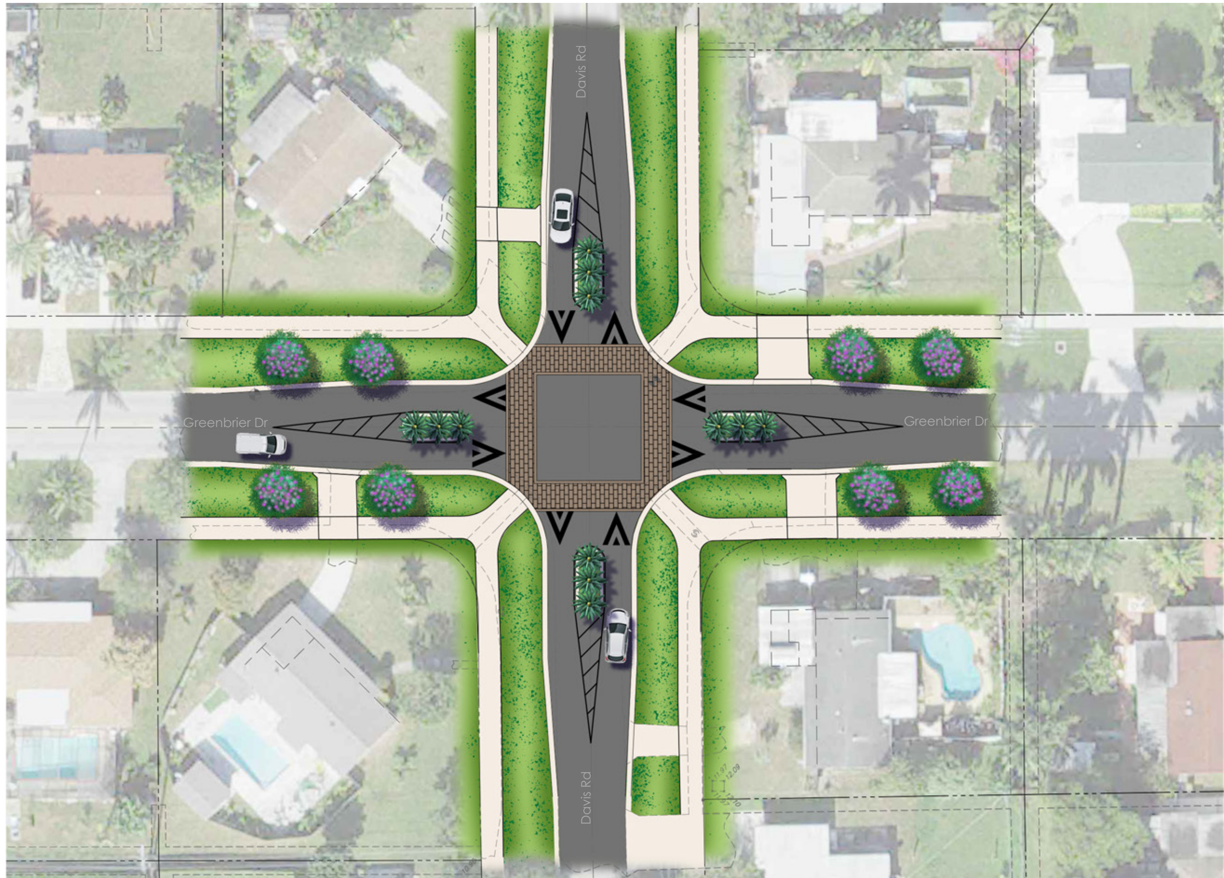
Greenbrier & Davis Intersection Plan View
